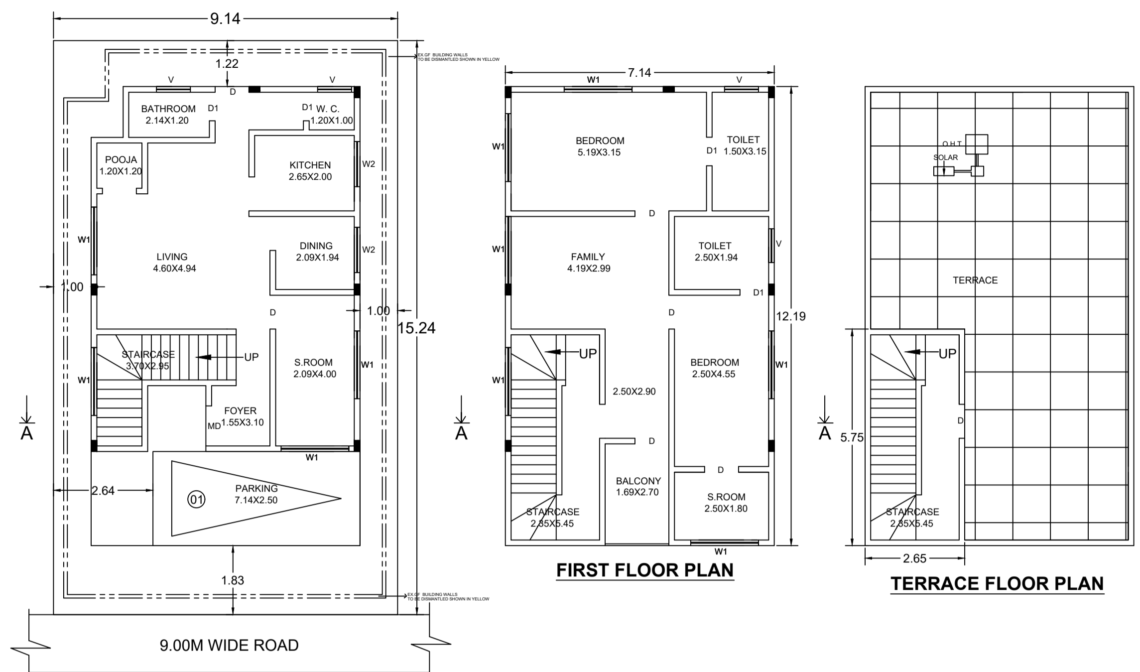
EX.GROUND FLOOR PLAN
